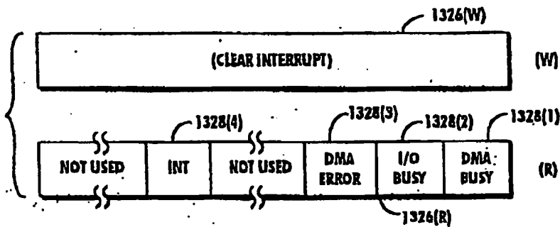
SI STATUS CONTROL REGISTER (R/W)
